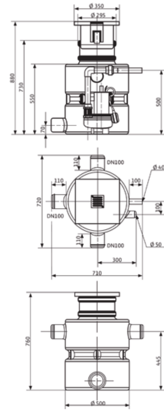
Wilo-DrainLift Box 40
