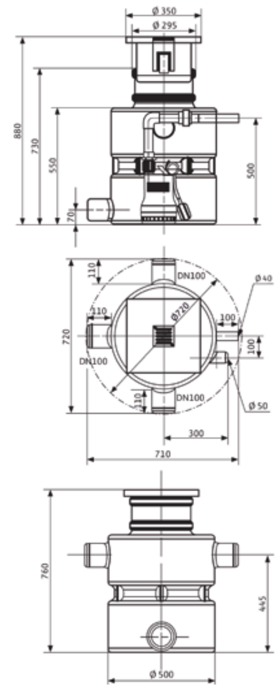
Wilo-DrainLift Box 32
